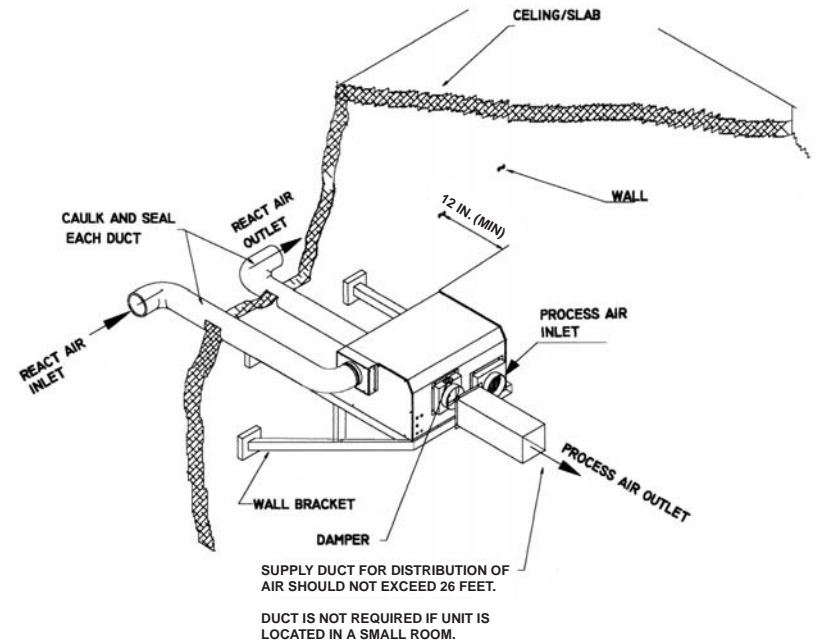
Wall mount installation
