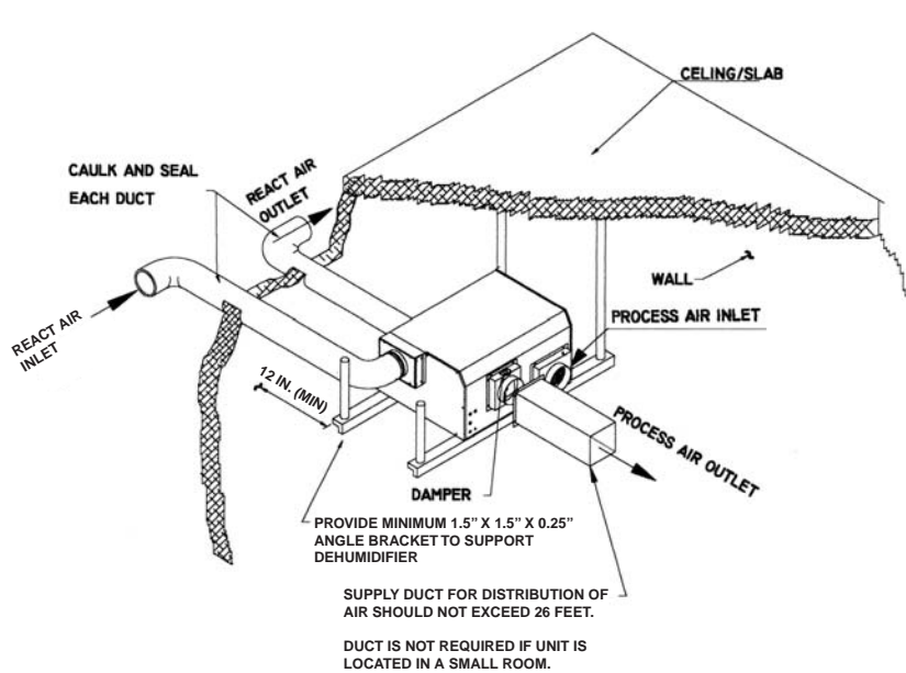
Ceiling mount installation
