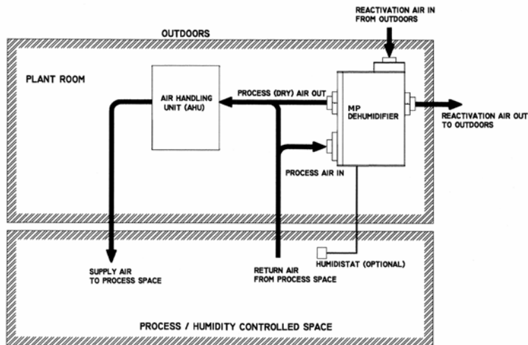
Installation with air handling unit
