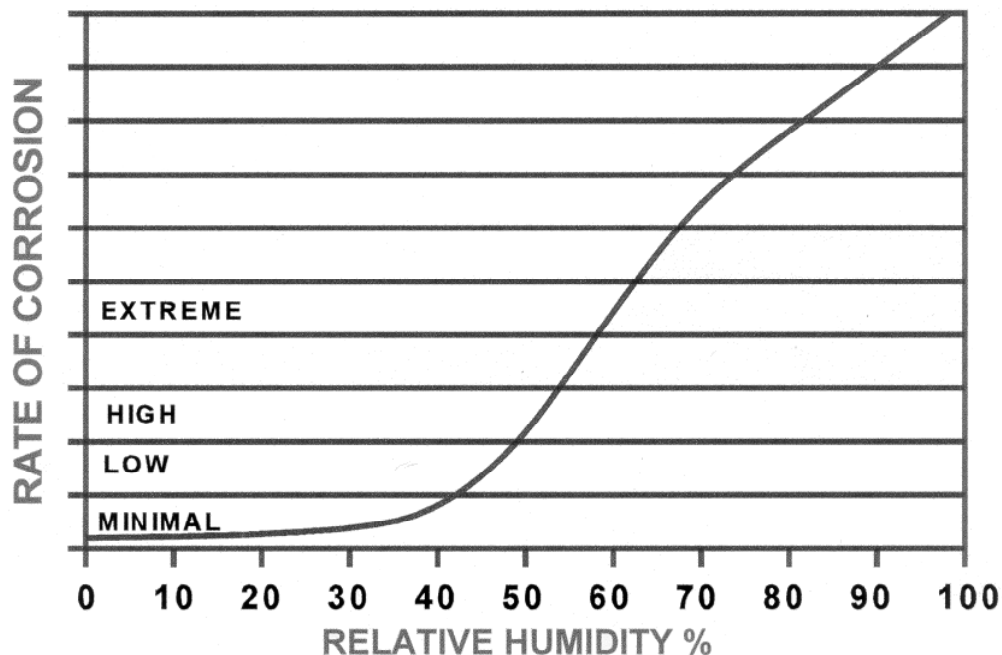
Typical Rate of Corrosion for Ferrous Metals
